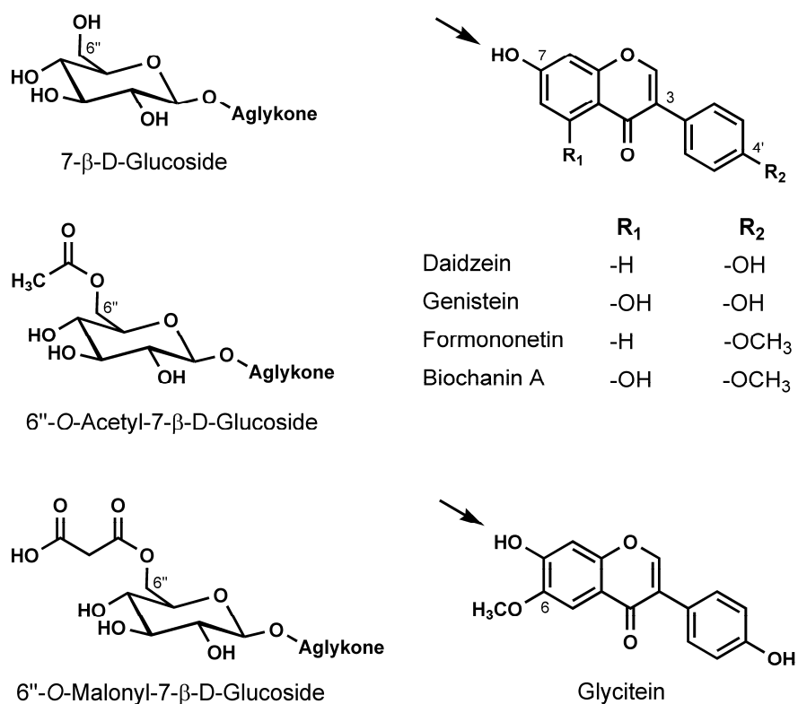
Fig. 1: Chemical structures of isoflavones in soy and red clover and their sugar conjugates. The 7-O-β-D-glucosides of daidzein, genistein and glycitein are known as daidzin, genistin and glycitin. The arrow in the Figure shows the position of sugar conjugation.
